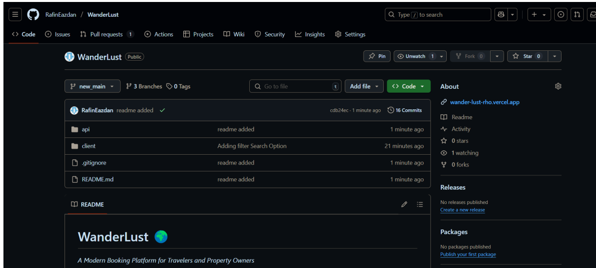
Figure 14: Github Repository
