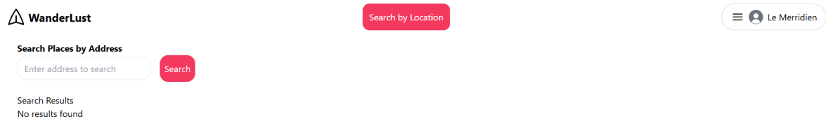
Figure 3: Search Page
