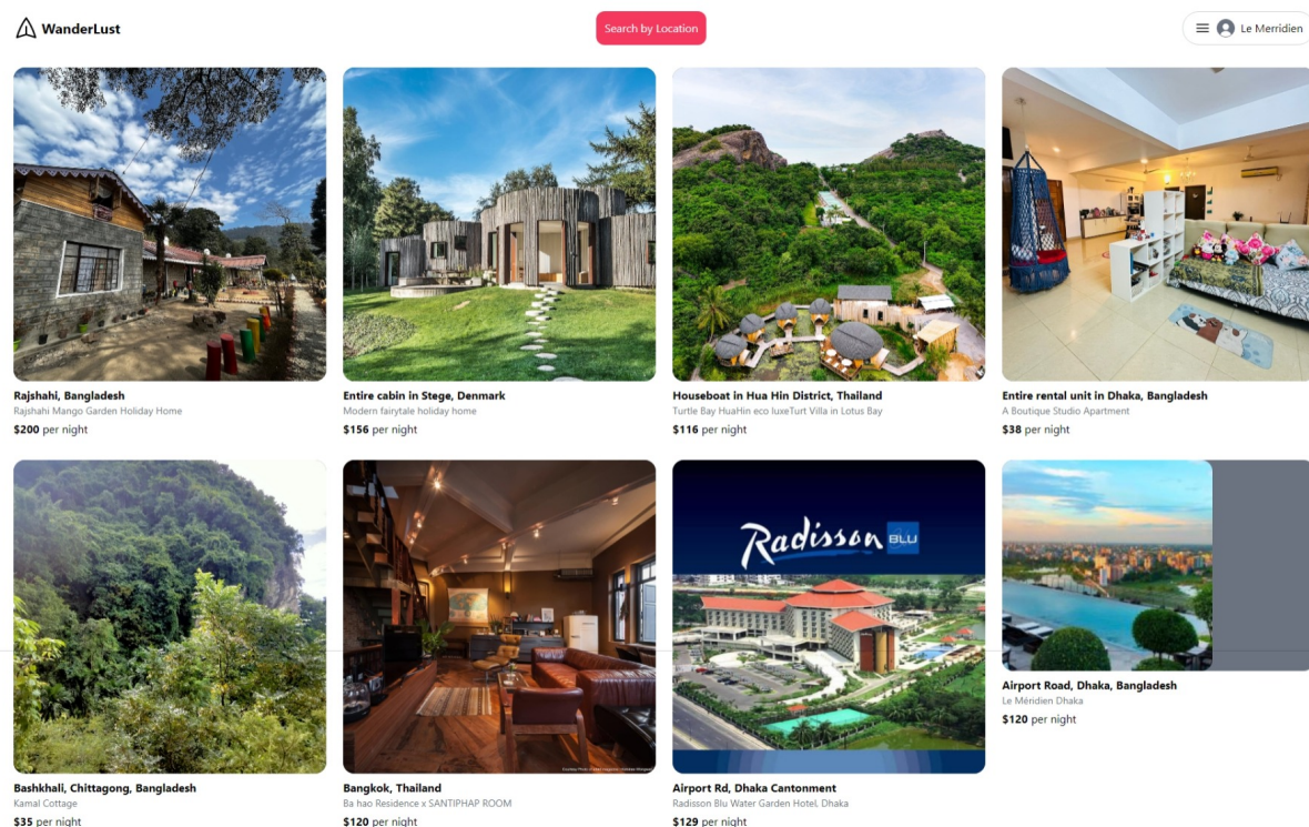
Figure 2: Home Page
